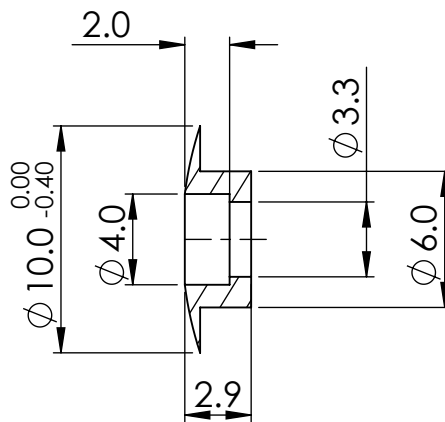
SECTION Y-Y
